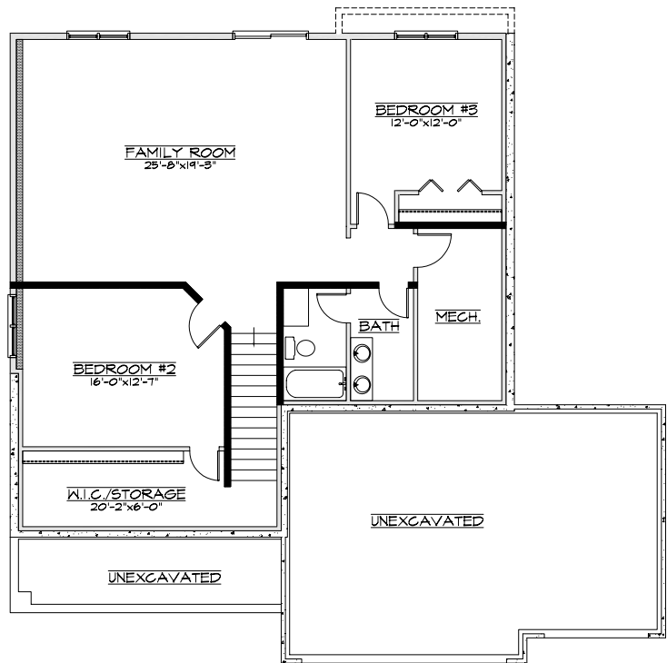
LOWER FLOOR PLAN
