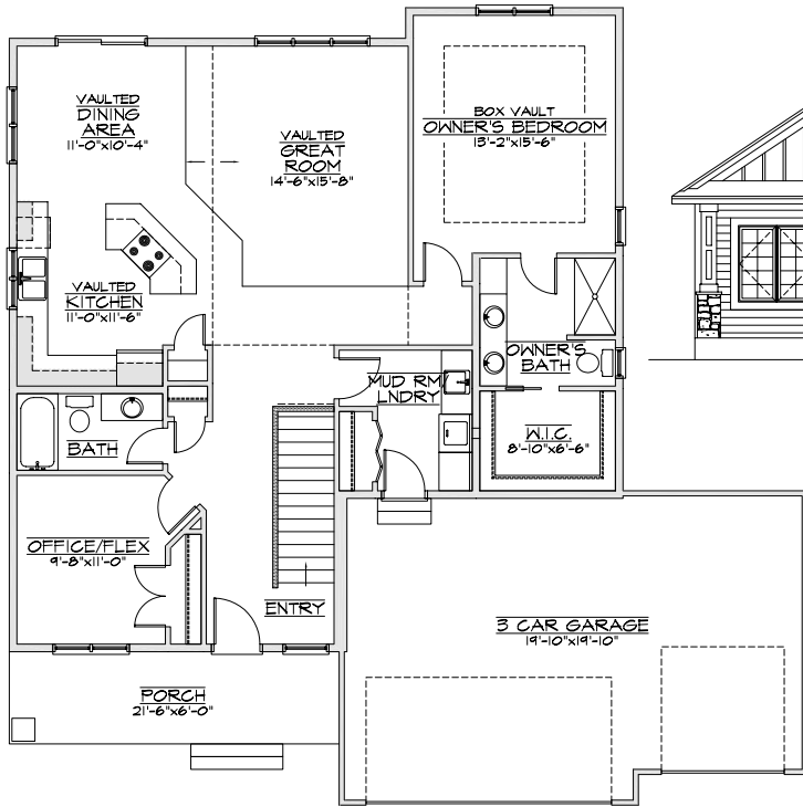
MAIN FLOOR PLAN 1448 SQ FT
